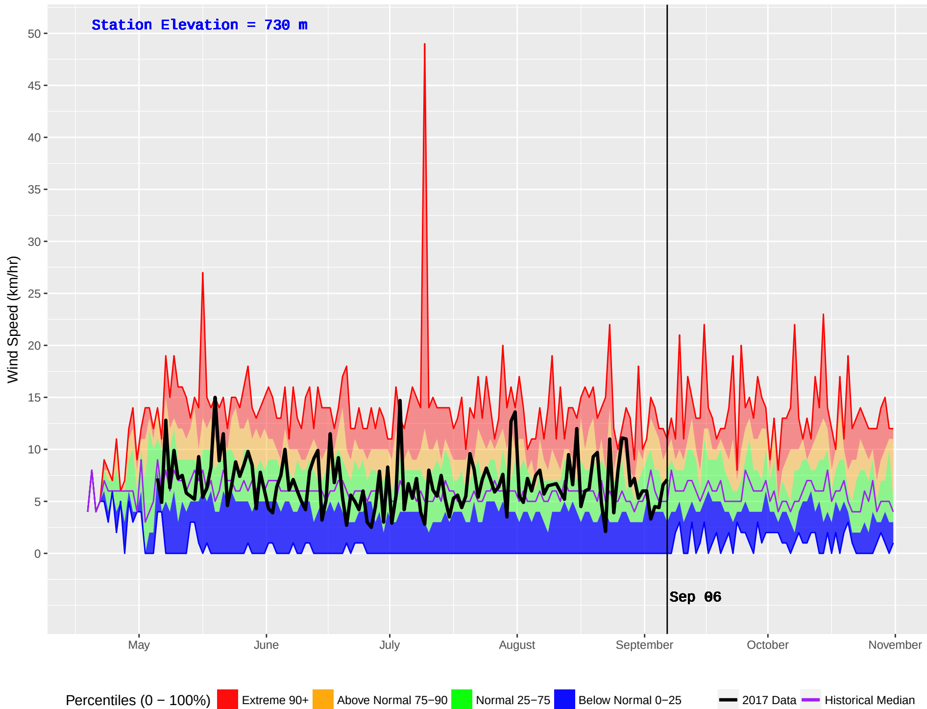
BOYA LAKE (445) : Historical (1985–2016) and Current (2017) Noon Wind Speed
