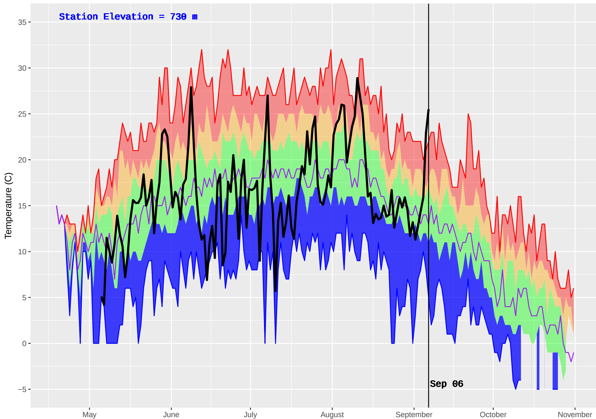
BOYA LAKE (445) : Historical (1985–2016) and Current (2017) Noon Temperature
