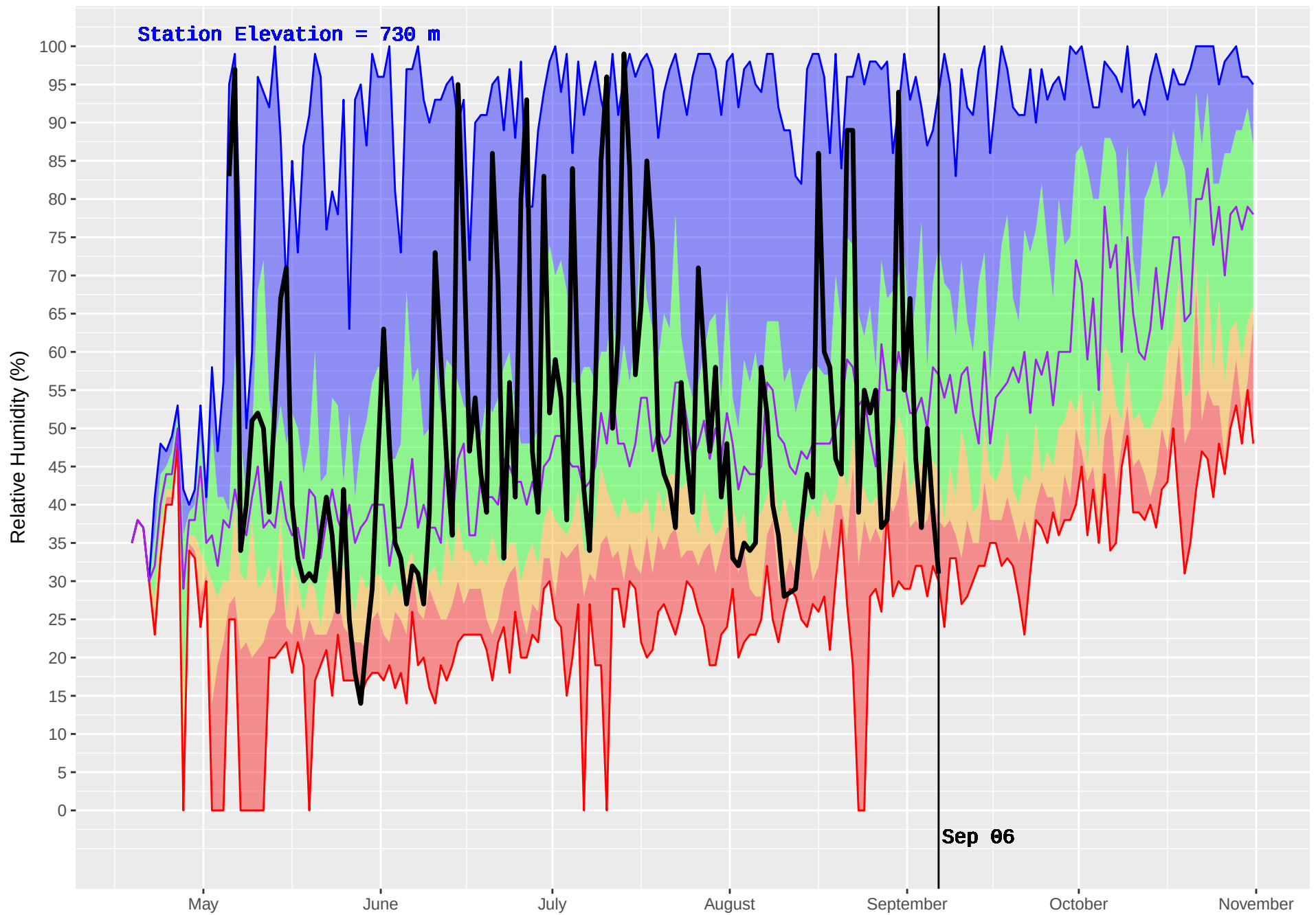
BOYA LAKE (445) : Historical (1985–2016) and Current (2017) Noon Relative Humidity
