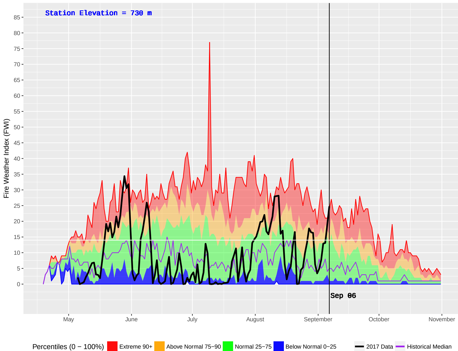
BOYA LAKE (445) : Historical (1985–2016) and Current (2017) Noon Fire Weather Index (FWI)
